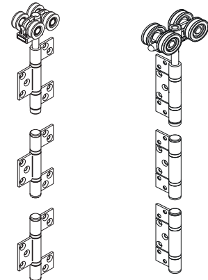
BWS4F-35CH
