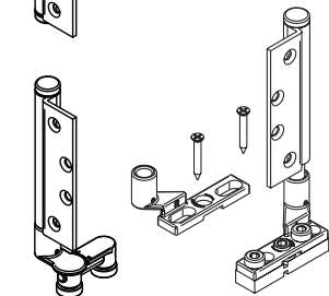
BWS2-100SM
